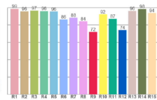
CRI: 92.6 (R1-R8)
